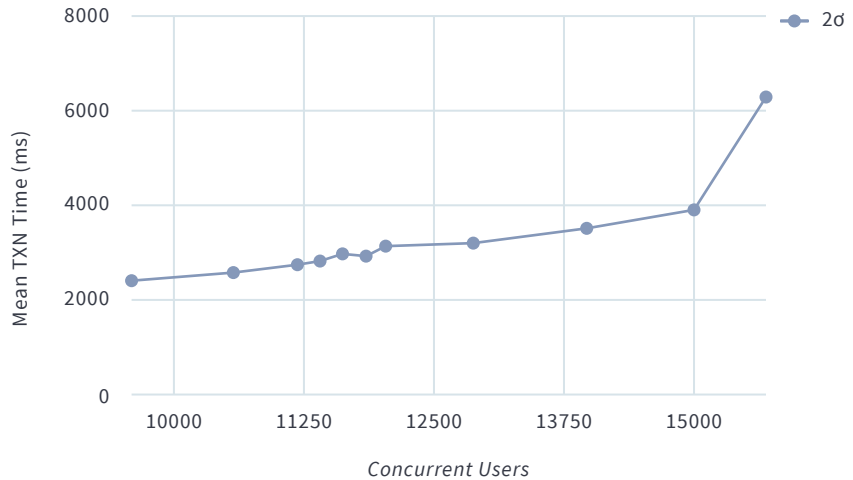
Figure 4: Legacy Login
