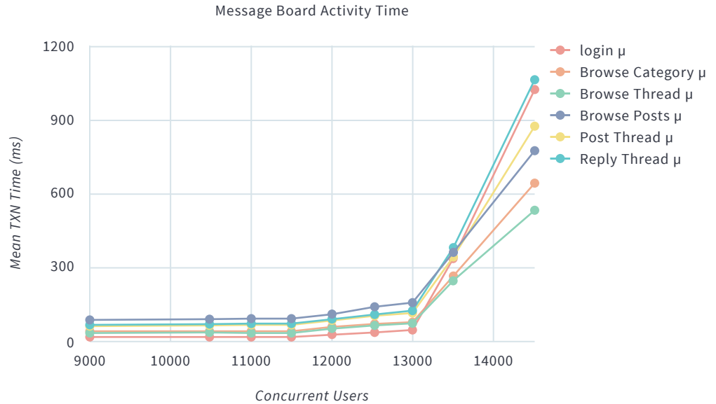
Figure 5: Collaboration Performance
